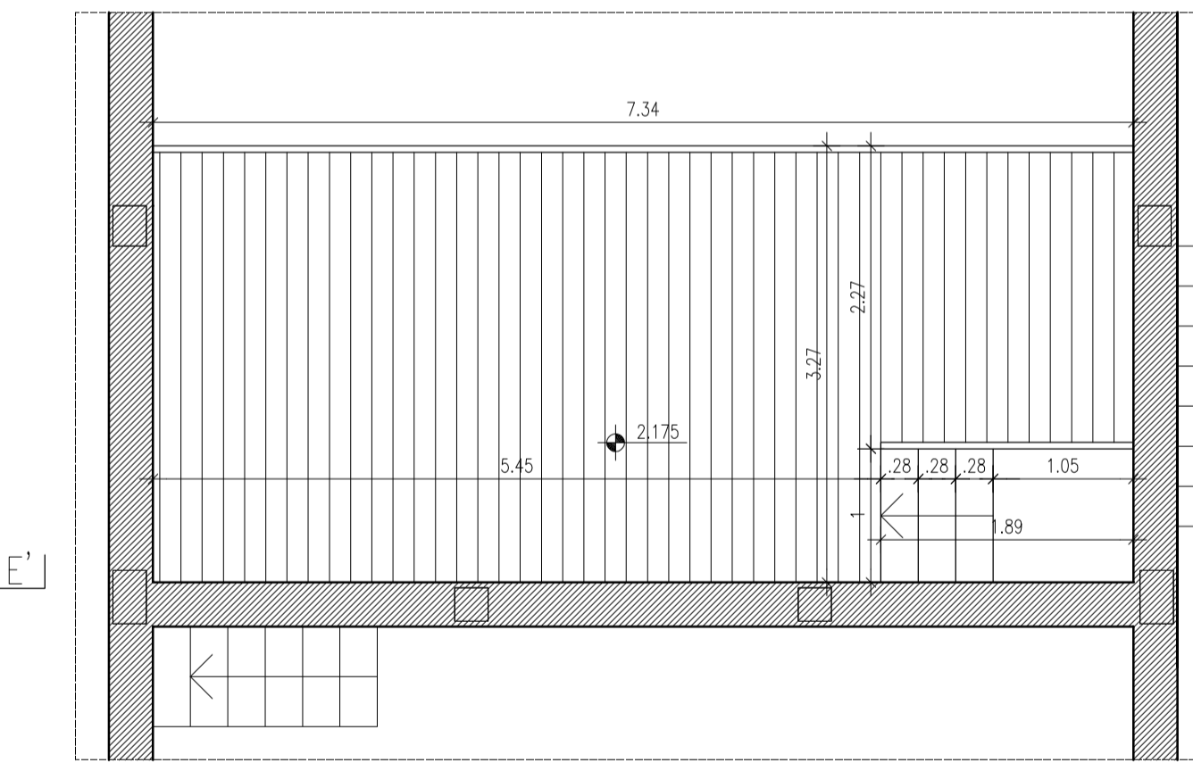
PLANTA MEZZANINE (COTA 4.10M)
